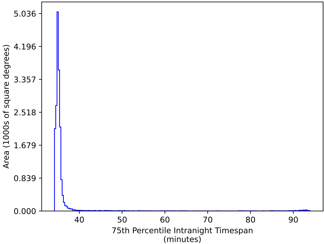
roll_pause_mjdp270_v3.4_10yrs WFD ri bands: 75th Percentile Intranight Timespan
