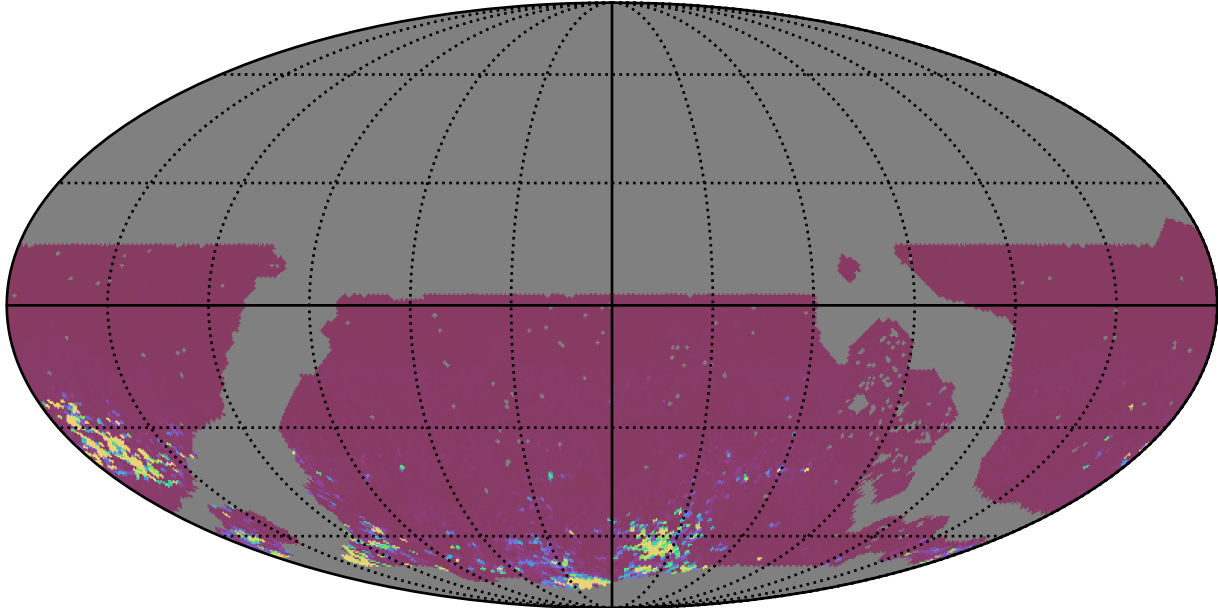
roll_pause_mjdp270_v3.4_10yrs WFD gr bands: 75th Percentile Intranight Timespan
