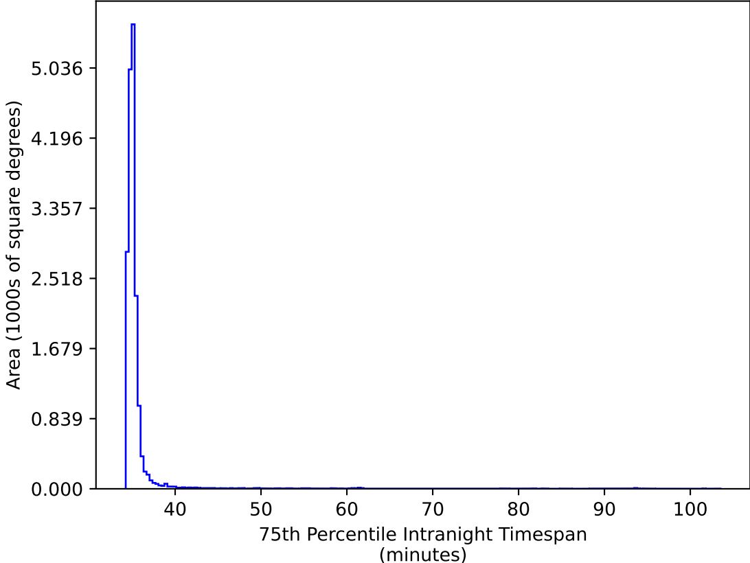
roll_pause_mjdp270_v3.4_10yrs WFD gr bands: 75th Percentile Intranight Timespan
