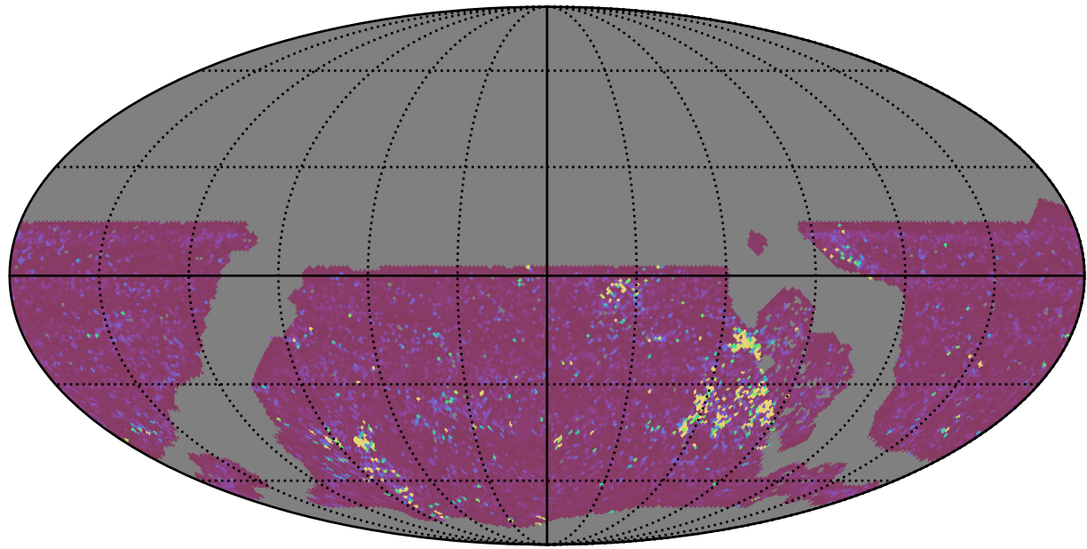
roll_pause_mjdp270_v3.4_10yrs WFD g band: 75th Percentile Intranight Timespan
