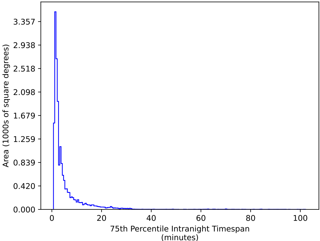
roll_pause_mjdp270_v3.4_10yrs WFD g band: 75th Percentile Intranight Timespan
