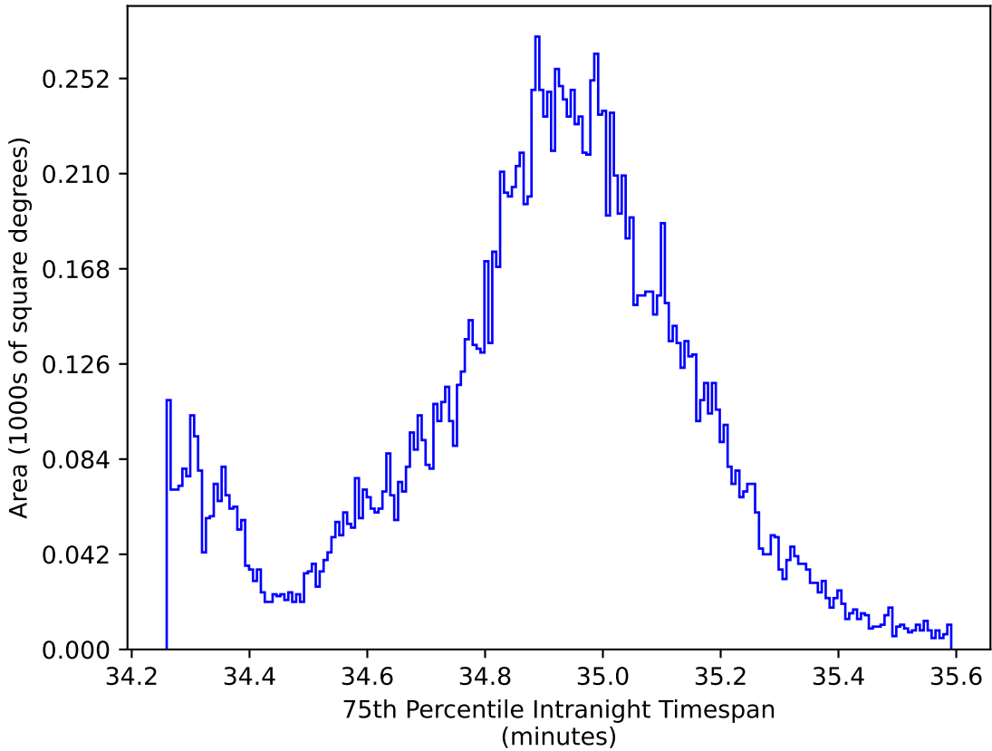
roll_pause_mjdp270_v3.4_10yrs WFD all bands: 75th Percentile Intranight Timespan
