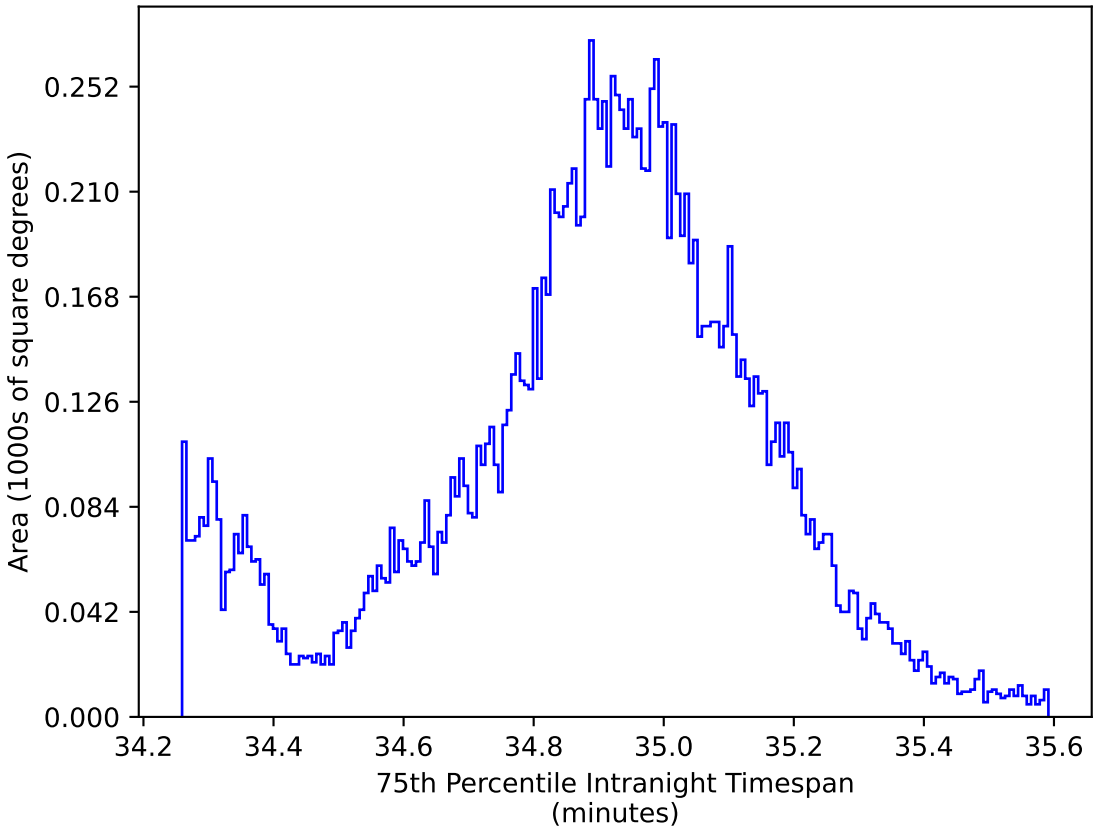
roll_pause_mjdp270_v3.4_10yrs WFD: 75th Percentile Intranight Timespan
