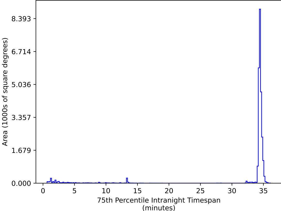
roll_pause_mjdp270_v3.4_10yrs All sky zy bands: 75th Percentile Intranight Timespan
