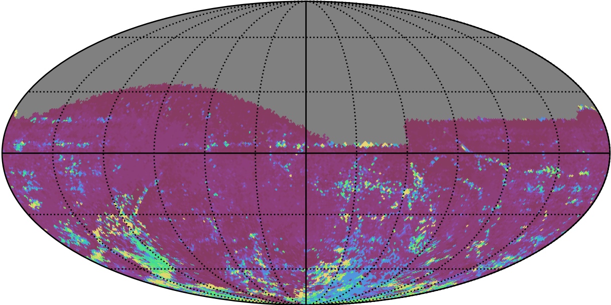
roll_pause_mjdp270_v3.4_10yrs All sky z band: 75th Percentile Intranight Timespan
