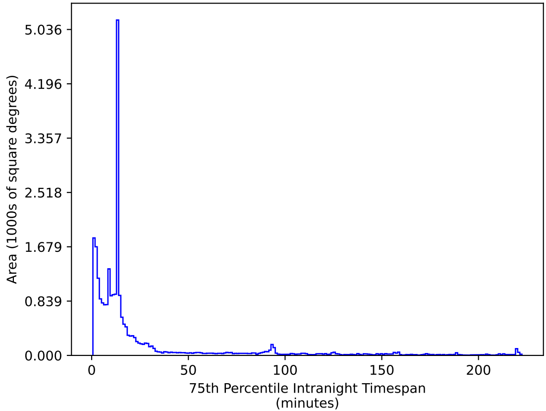
roll_pause_mjdp270_v3.4_10yrs All sky z band: 75th Percentile Intranight Timespan
