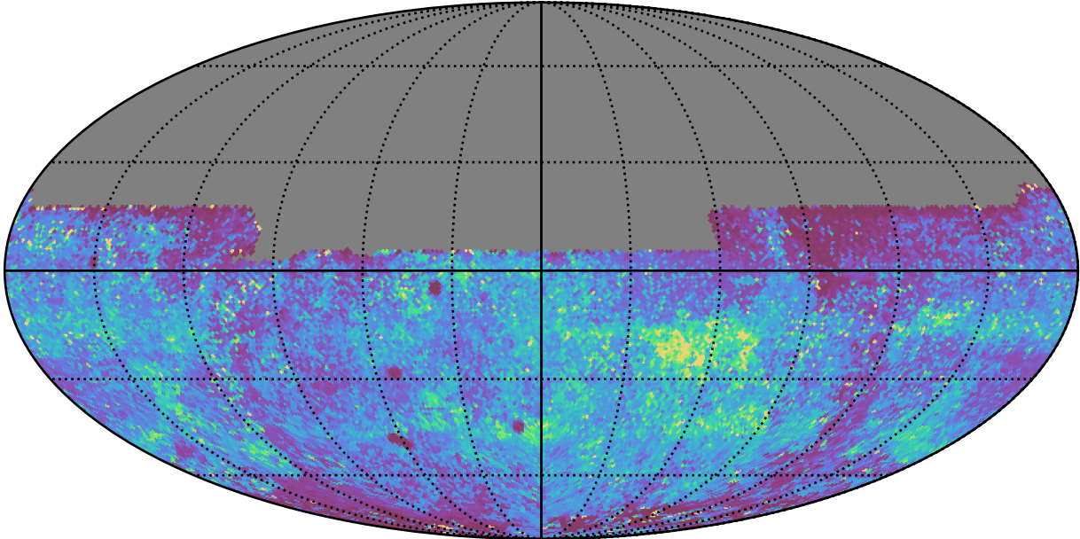
roll_pause_mjdp270_v3.4_10yrs All sky y band: 75th Percentile Intranight Timespan
