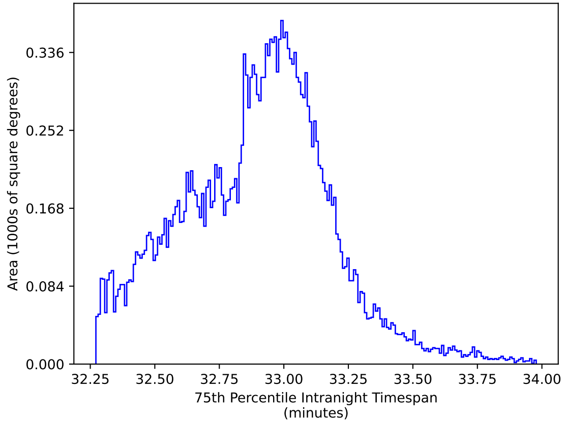
roll_pause_mjdp270_v3.4_10yrs All sky y band: 75th Percentile Intranight Timespan
