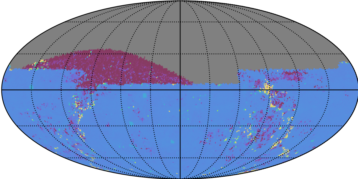
roll_pause_mjdp270_v3.4_10yrs All sky ug bands: 75th Percentile Intranight Timespan
