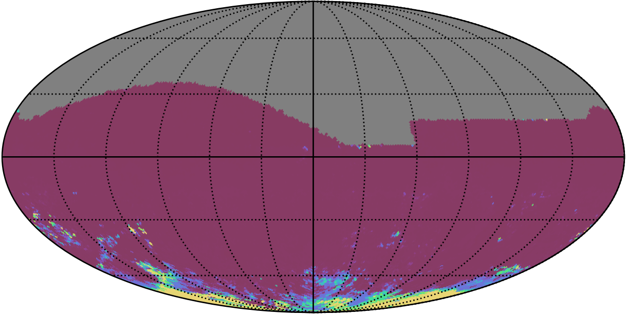
roll_pause_mjdp270_v3.4_10yrs All sky ri bands: 75th Percentile Intranight Timespan
