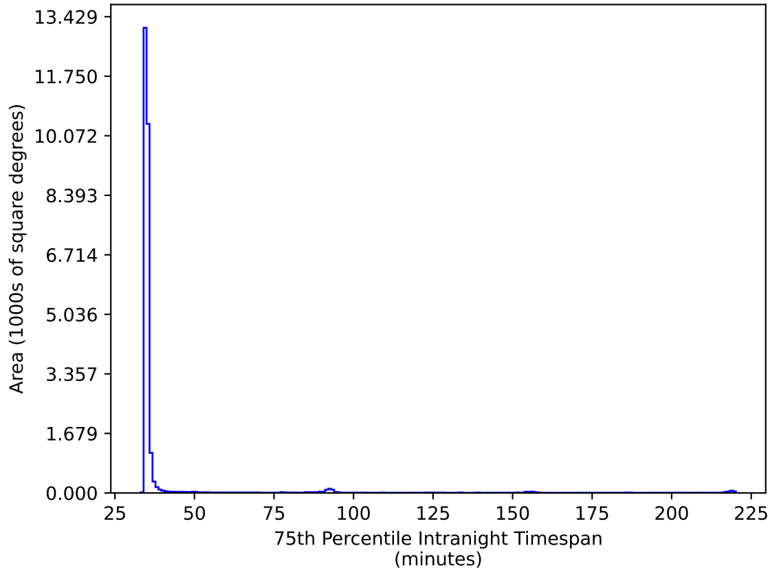
roll_pause_mjdp270_v3.4_10yrs All sky ri bands: 75th Percentile Intranight Timespan
