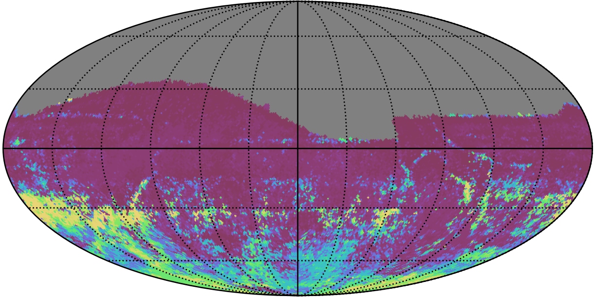
roll_pause_mjdp270_v3.4_10yrs All sky r band: 75th Percentile Intranight Timespan
