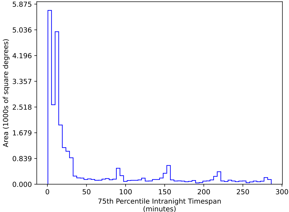
roll_pause_mjdp270_v3.4_10yrs All sky r band: 75th Percentile Intranight Timespan
