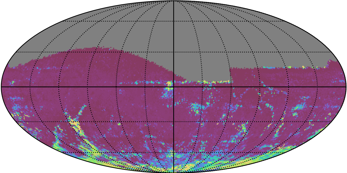
roll_pause_mjdp270_v3.4_10yrs All sky i band: 75th Percentile Intranight Timespan
