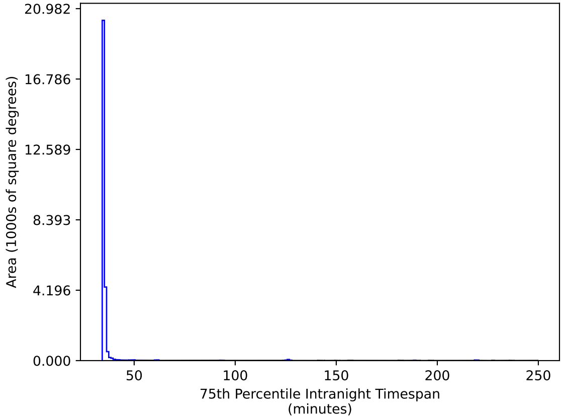
roll_pause_mjdp270_v3.4_10yrs All sky gr bands: 75th Percentile Intranight Timespan
