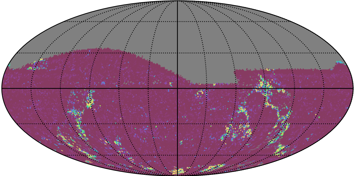
roll_pause_mjdp270_v3.4_10yrs All sky g band: 75th Percentile Intranight Timespan
