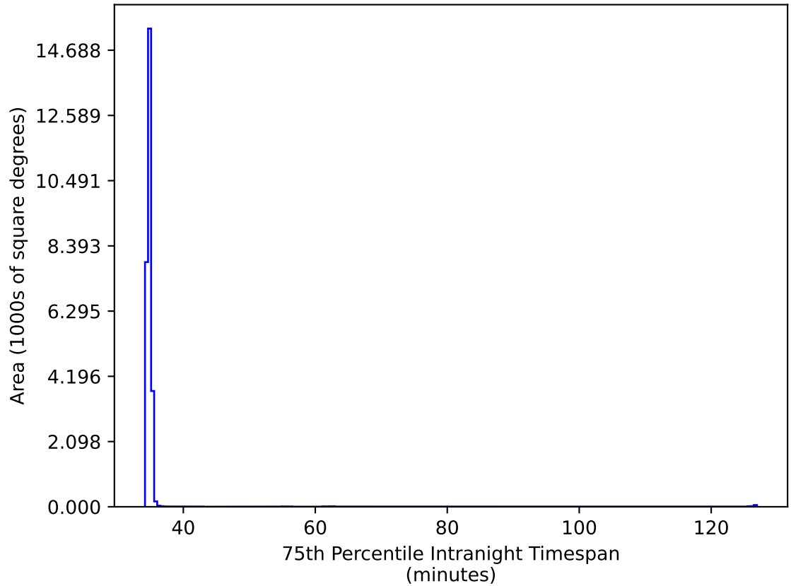
roll_pause_mjdp270_v3.4_10yrs All sky all bands: 75th Percentile Intranight Timespan
