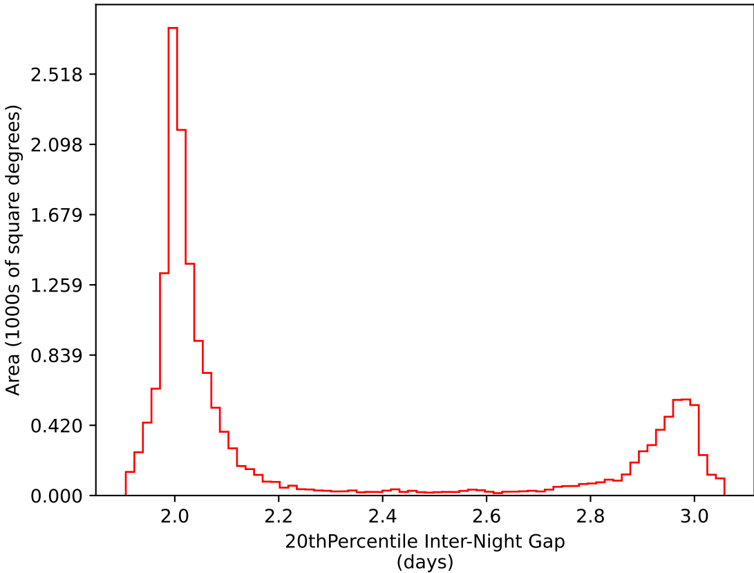
roll_pause_mjdp270_v3.4_10yrs WFD i band: 20thPercentile Inter-Night Gap
