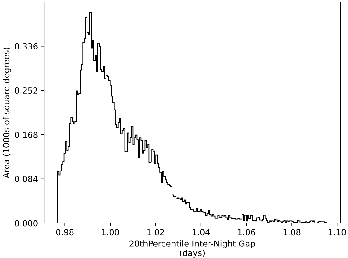
roll_pause_mjdp270_v3.4_10yrs WFD all bands: 20thPercentile Inter-Night Gap
