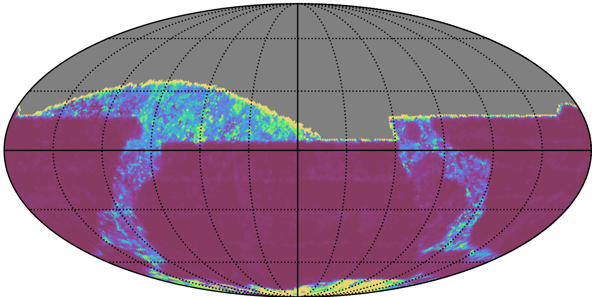
roll_pause_mjdp270_v3.4_10yrs All sky z band: 20thPercentile Inter-Night Gap
