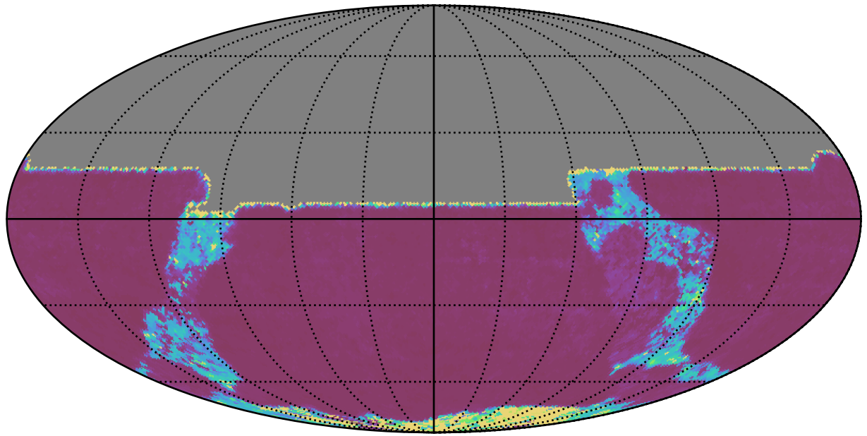
roll_pause_mjdp270_v3.4_10yrs All sky y band: 20thPercentile Inter-Night Gap
