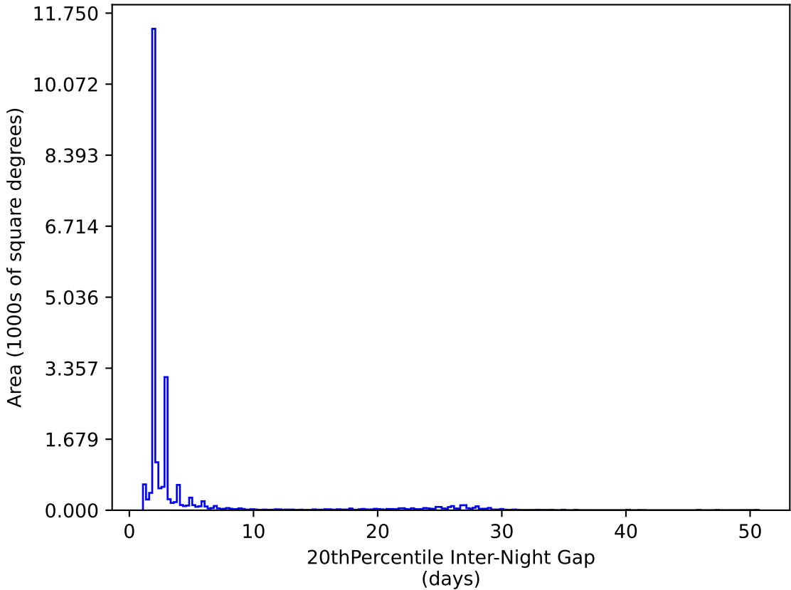
roll_pause_mjdp270_v3.4_10yrs All sky y band: 20thPercentile Inter-Night Gap
