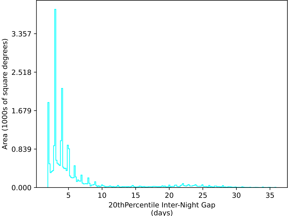
roll_pause_mjdp270_v3.4_10yrs All sky u band: 20thPercentile Inter-Night Gap
