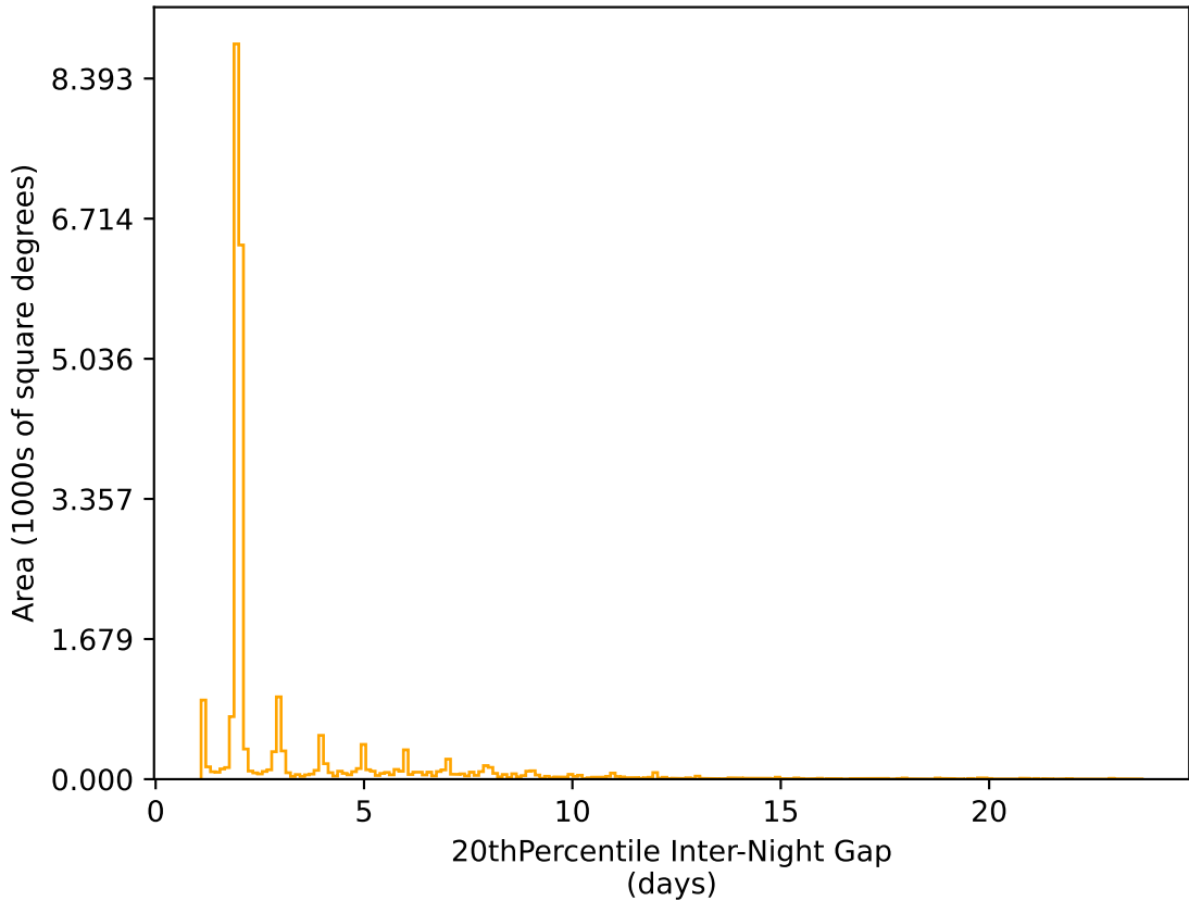
roll_pause_mjdp270_v3.4_10yrs All sky r band: 20thPercentile Inter-Night Gap
