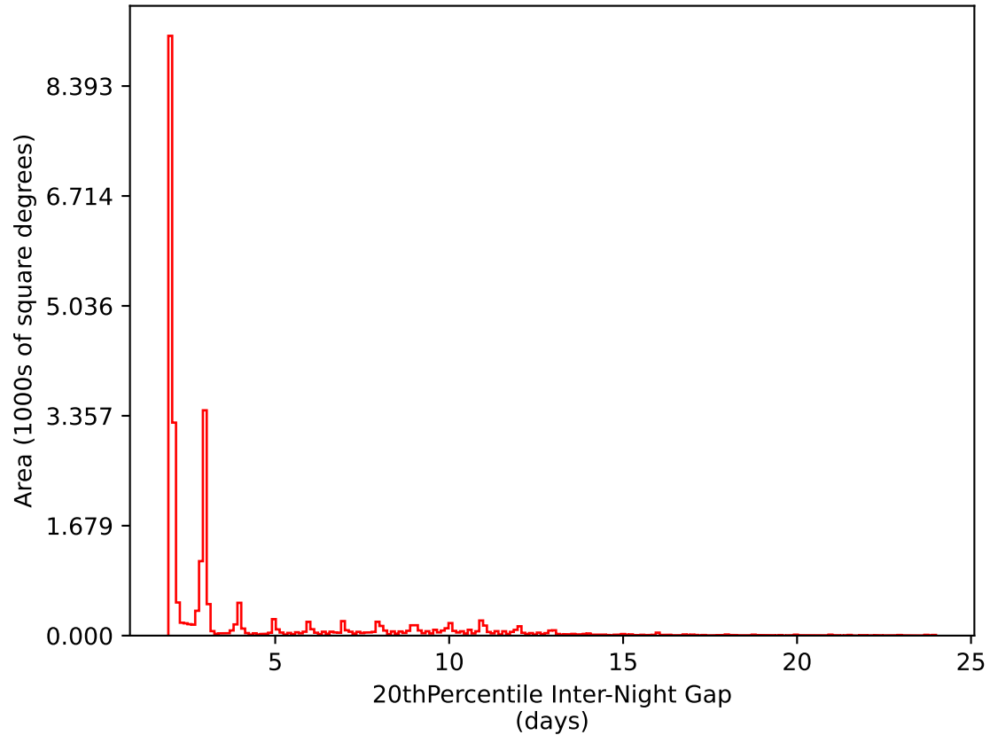
roll_pause_mjdp270_v3.4_10yrs All sky i band: 20thPercentile Inter-Night Gap
