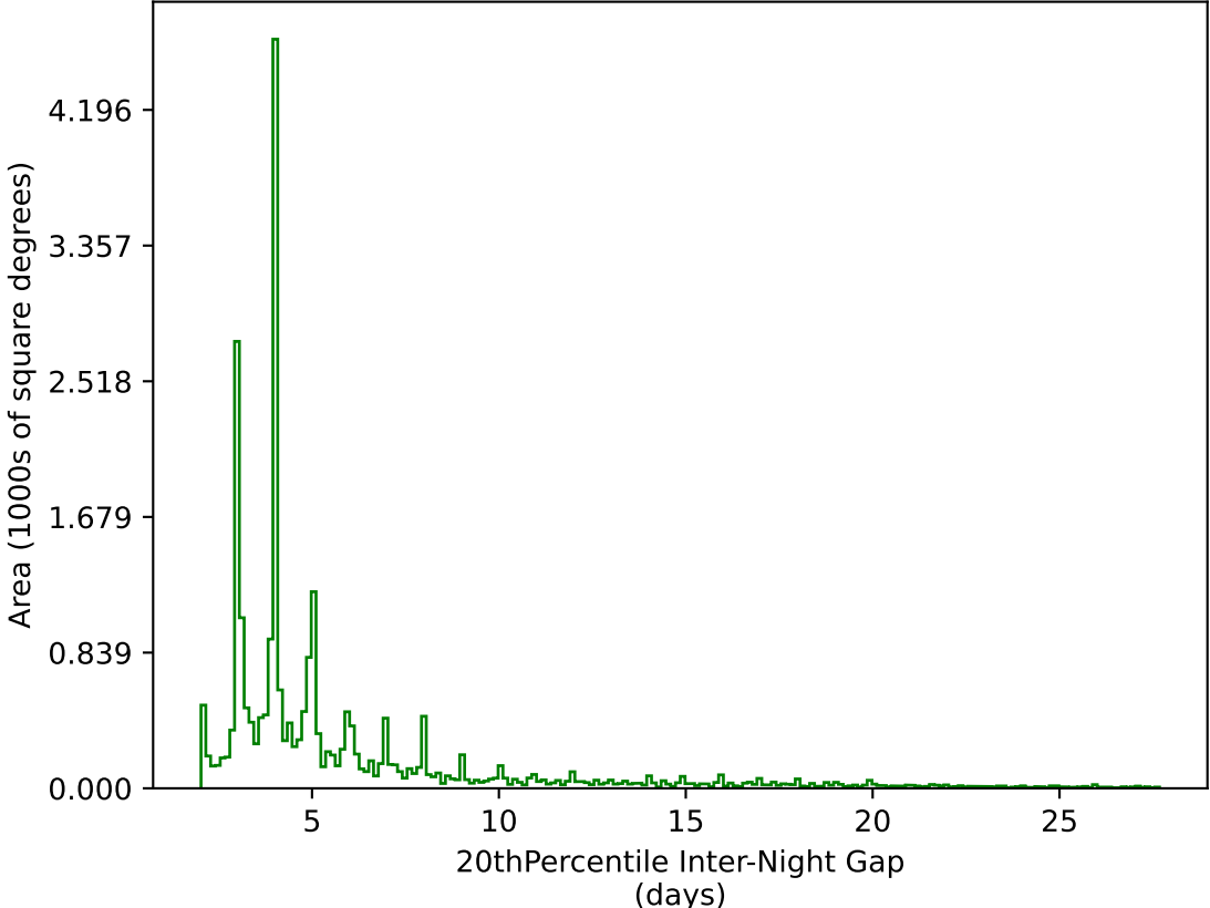
roll_pause_mjdp270_v3.4_10yrs All sky g band: 20thPercentile Inter-Night Gap
