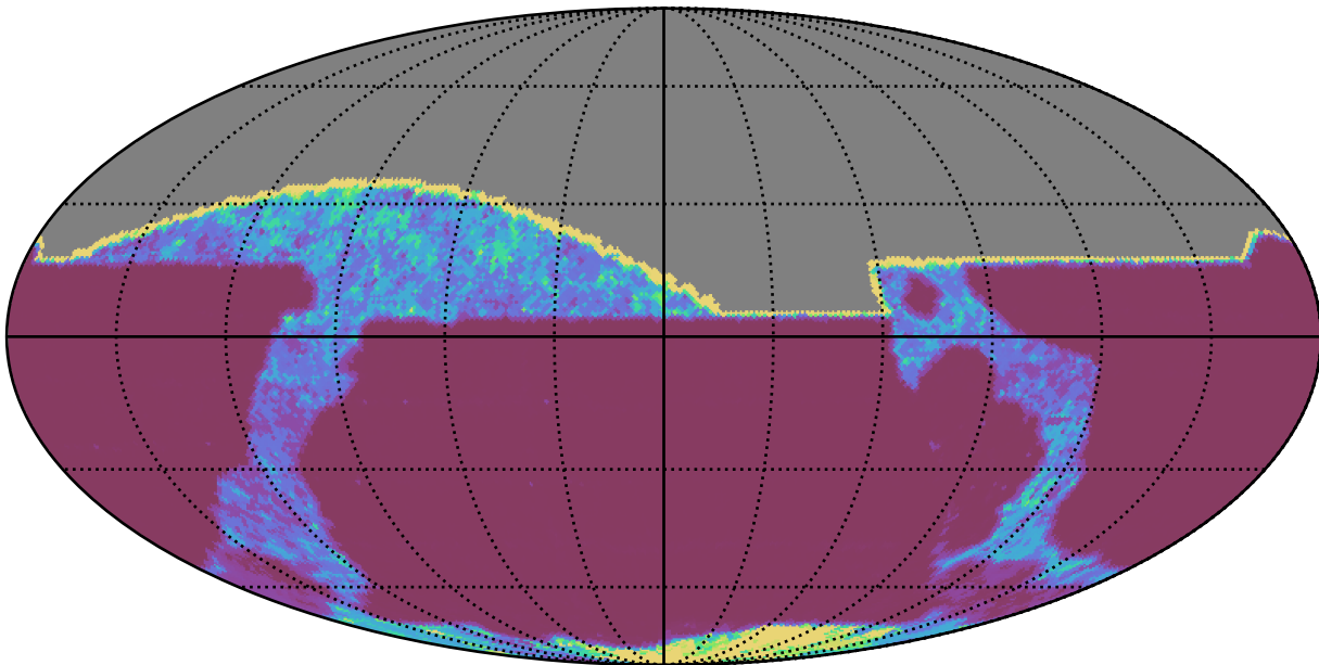
roll_pause_mjdp270_v3.4_10yrs All sky all bands: 20thPercentile Inter-Night Gap
