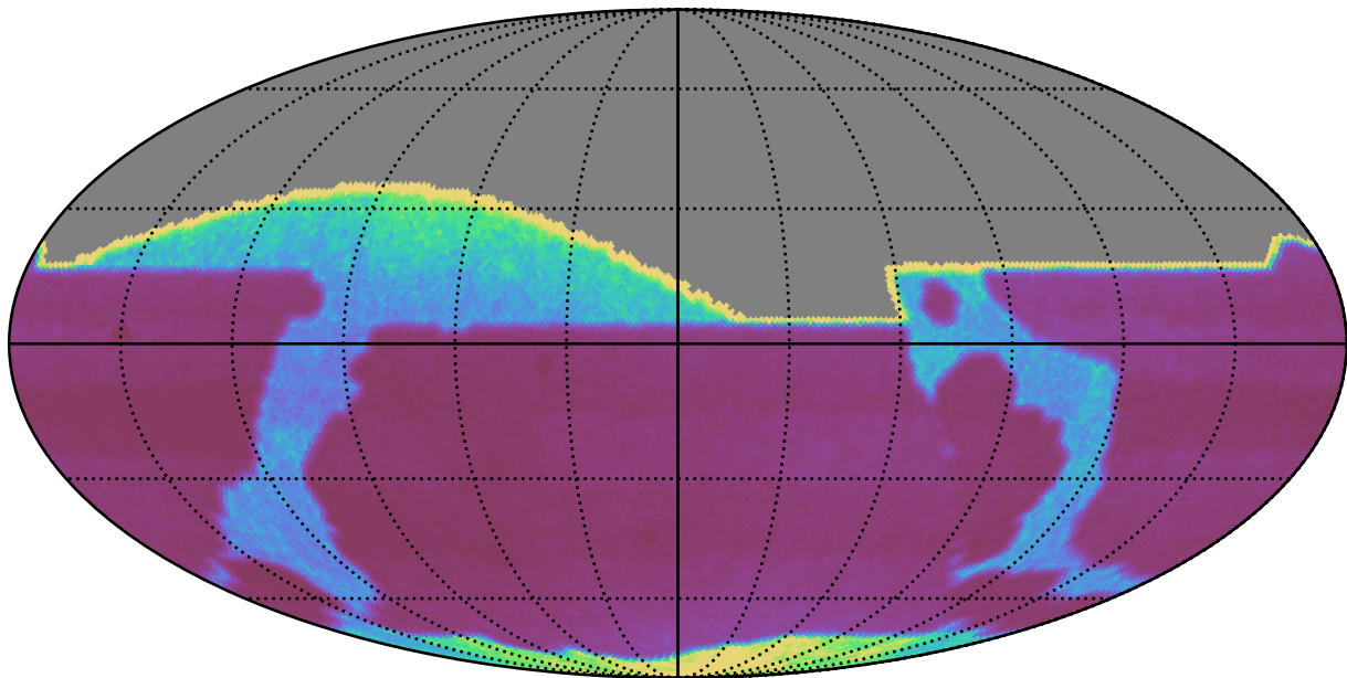
roll_pause_mjdp270_v3.4_10yrs : properMotion
