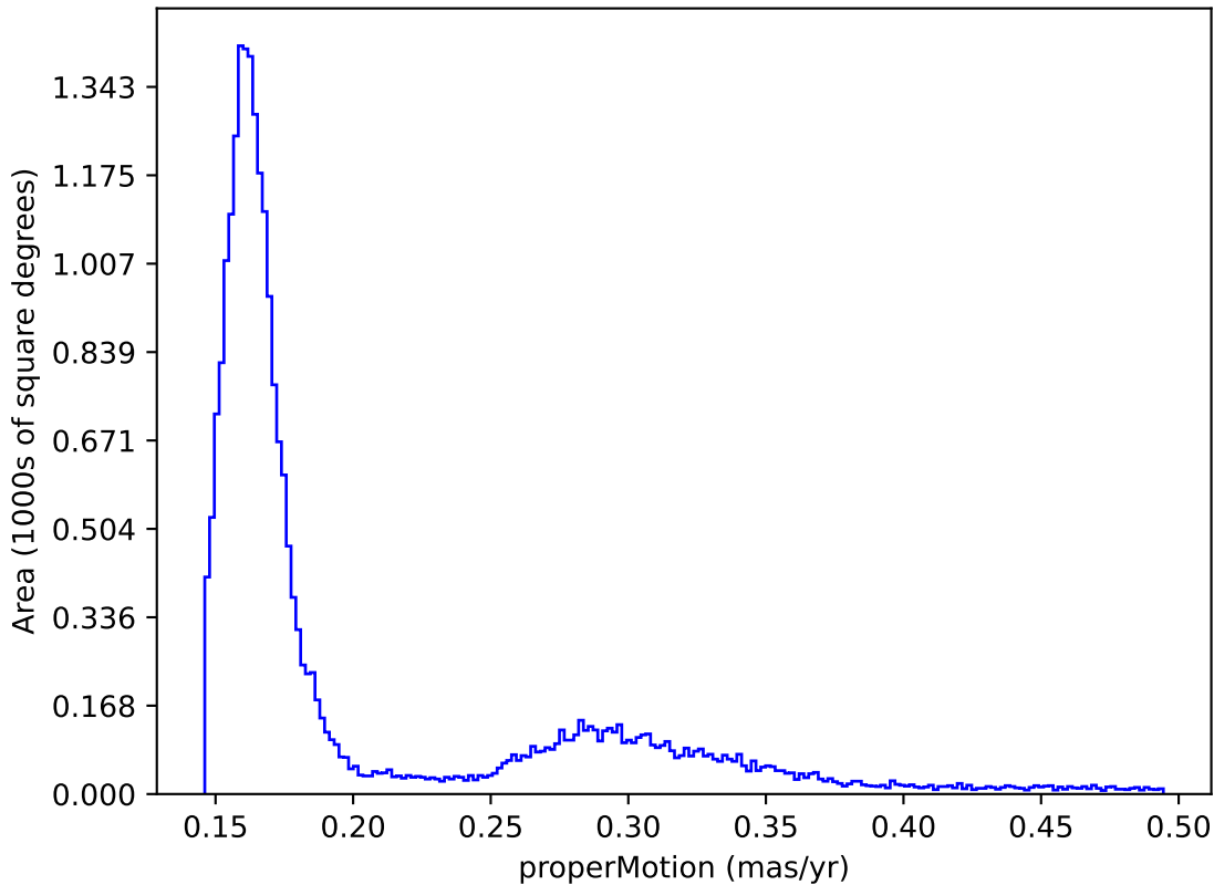
roll_pause_mjdp270_v3.4_10yrs : properMotion
