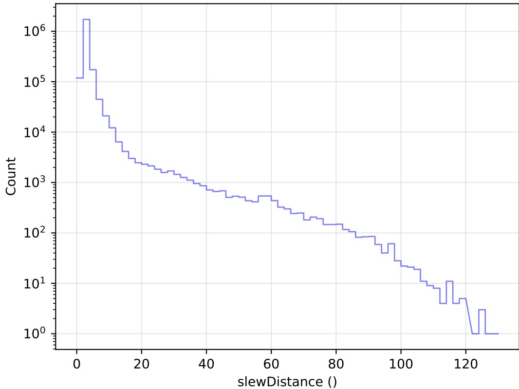
roll_pause_mjdp270_v3.4_10yrs All visits: Slew Distance Histogram
