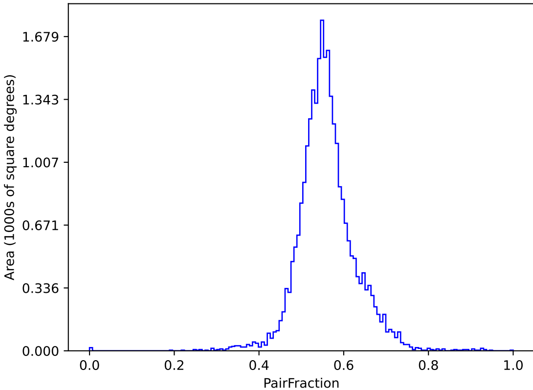
roll_pause_mjdp270_v3.4_10yrs (g or r or i): PairFraction
