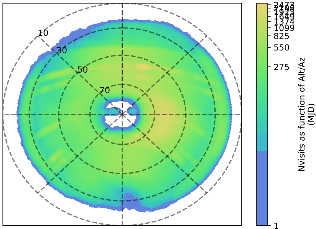
roll_pause_mjdp270_v3.4_10yrs z: Nvisits as function of Alt/Az
