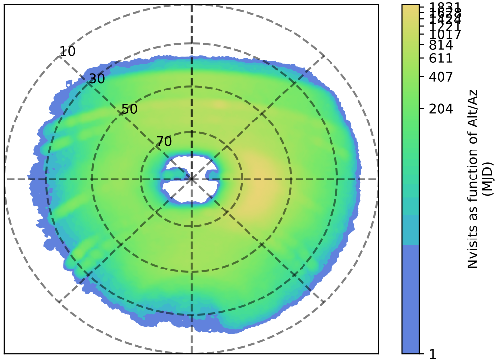
roll_pause_mjdp270_v3.4_10yrs y: Nvisits as function of Alt/Az
