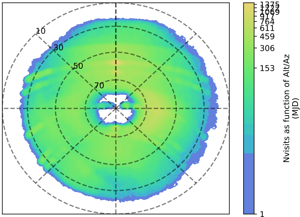
roll_pause_mjdp270_v3.4_10yrs g: Nvisits as function of Alt/Az
