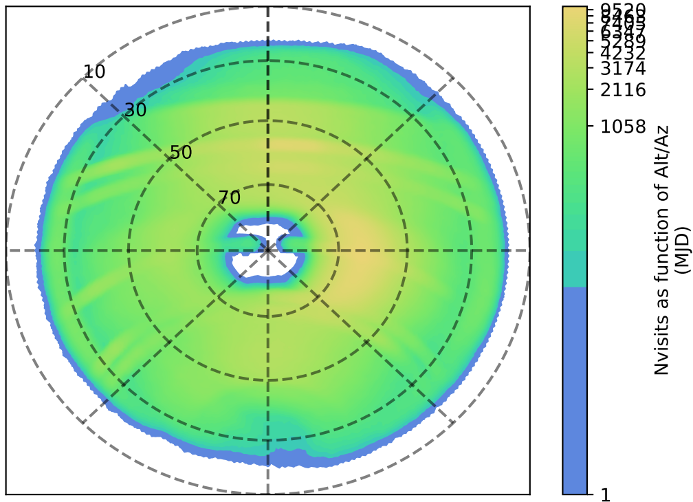
roll_pause_mjdp270_v3.4_10yrs : Nvisits as function of Alt/Az
