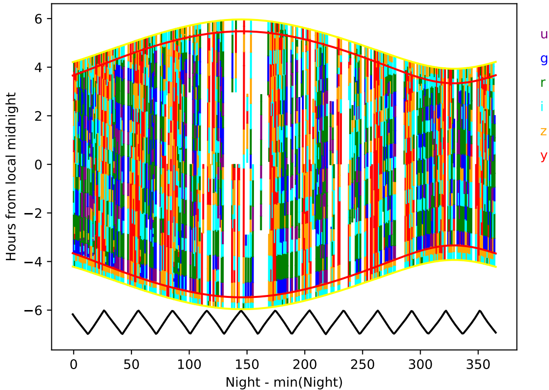
roll_pause_mjdp270_v3.4_10yrs year 9-10: Hourglass
