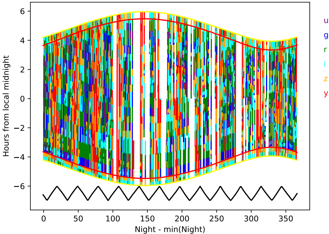
roll_pause_mjdp270_v3.4_10yrs year 7-8: Hourglass
