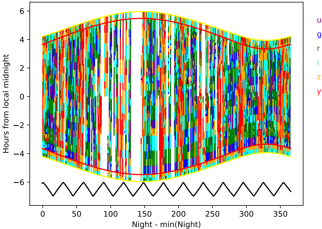
roll_pause_mjdp270_v3.4_10yrs year 6-7: Hourglass
