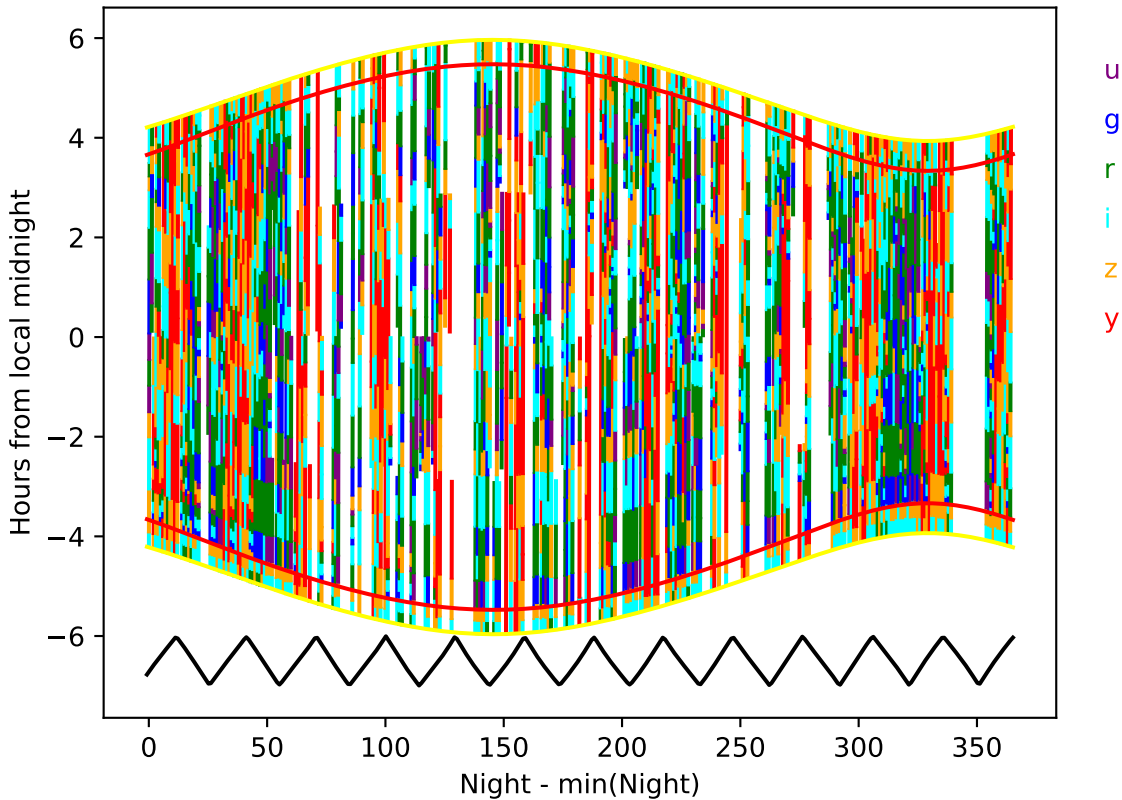
roll_pause_mjdp270_v3.4_10yrs year 5-6: Hourglass
