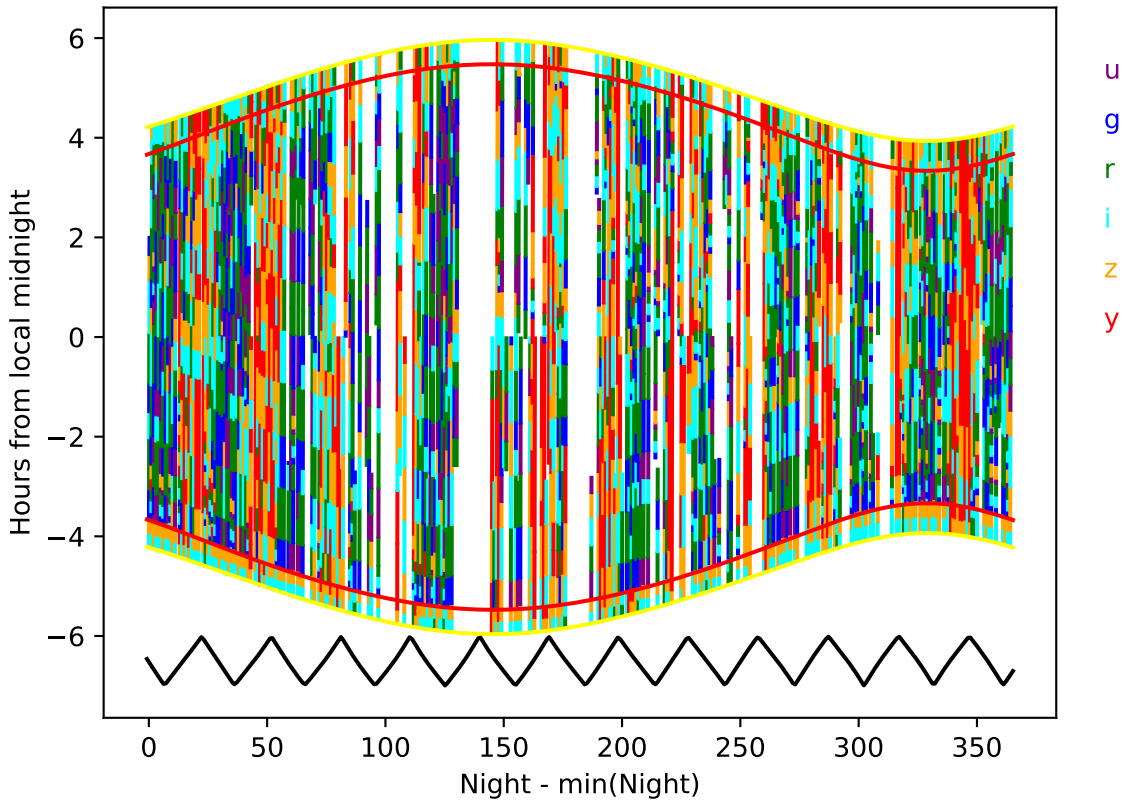
roll_pause_mjdp270_v3.4_10yrs year 4-5: Hourglass
