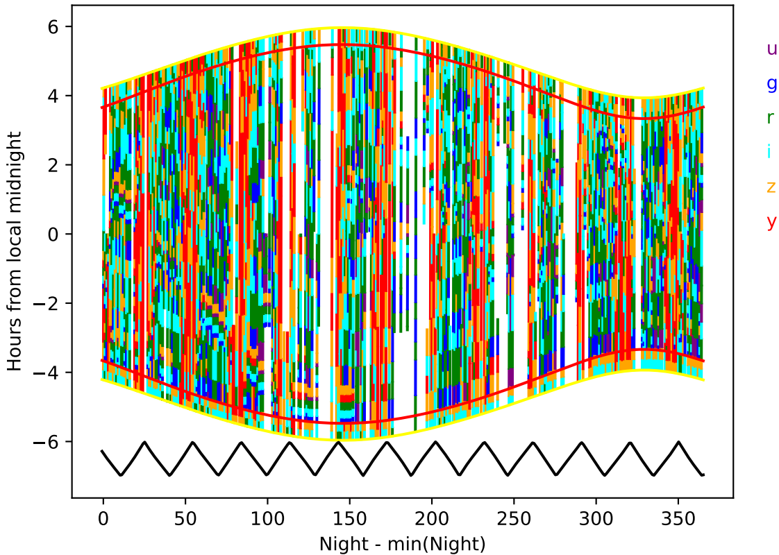
roll_pause_mjdp270_v3.4_10yrs year 1-2: Hourglass
