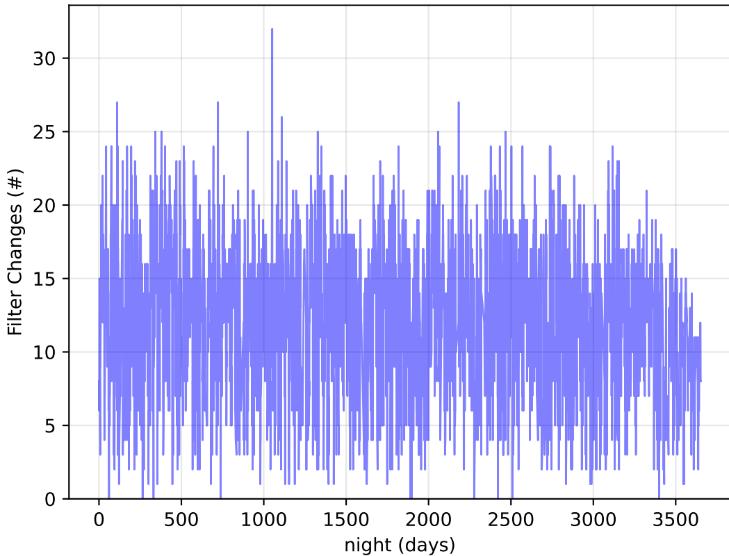
roll_pause_mjdp270_v3.4_10yrs : Filter Changes
