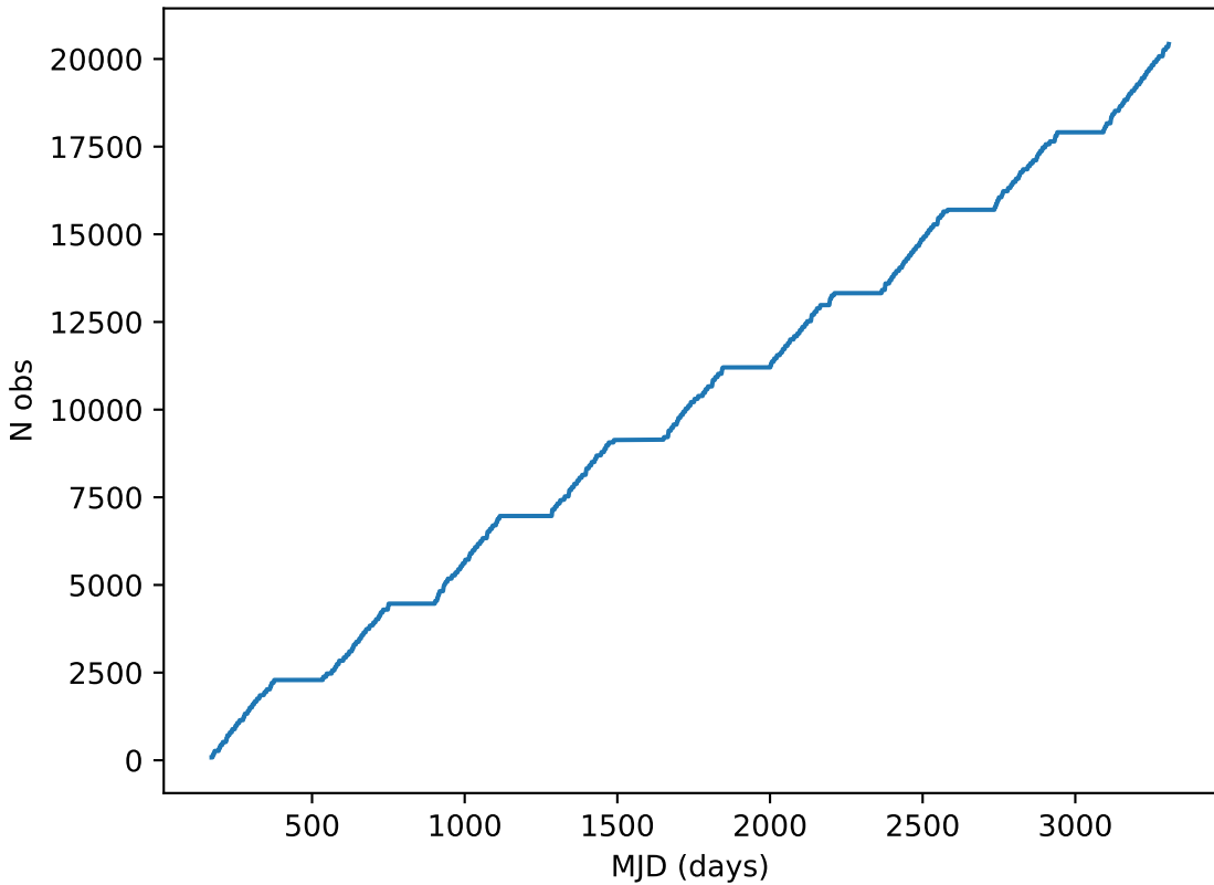
roll_pause_mjdp270_v3.4_10yrs note like DD:XMM_LSS%: Cumulative
