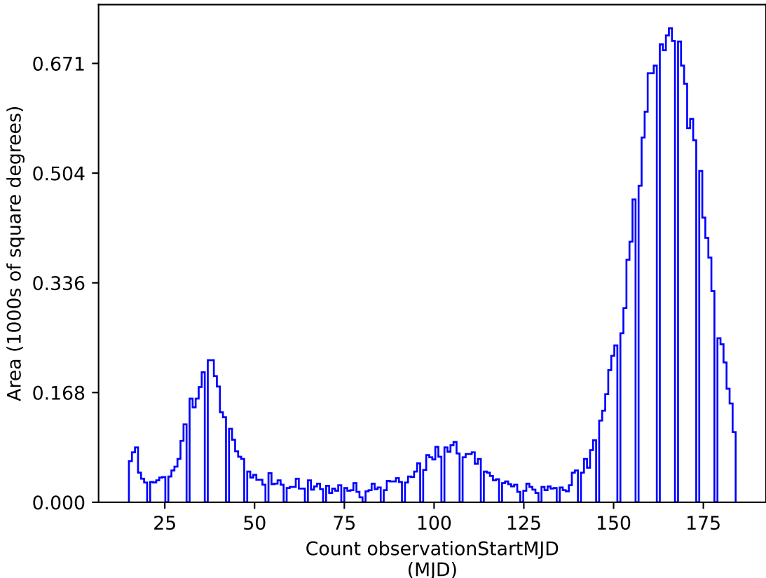
roll_pause_mjdp270_v3.4_10yrs y: Count observationStartMJD
