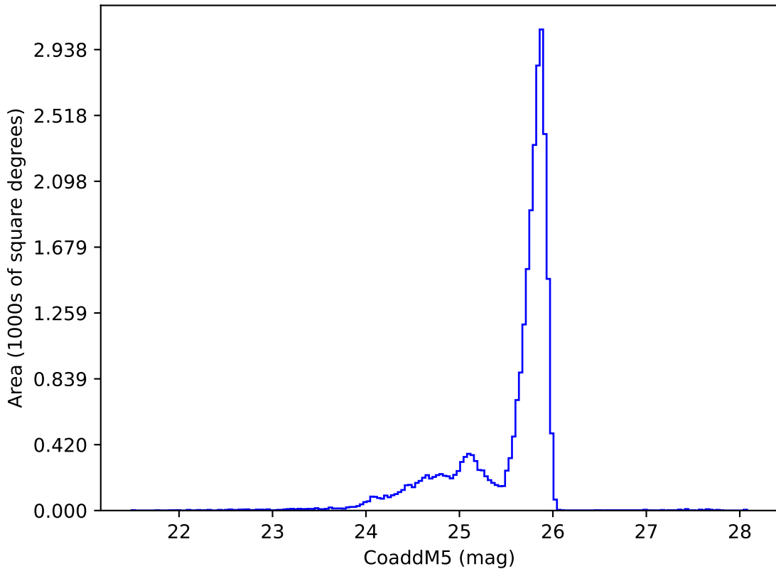
roll_pause_mjdp270_v3.4_10yrs z: CoaddM5
