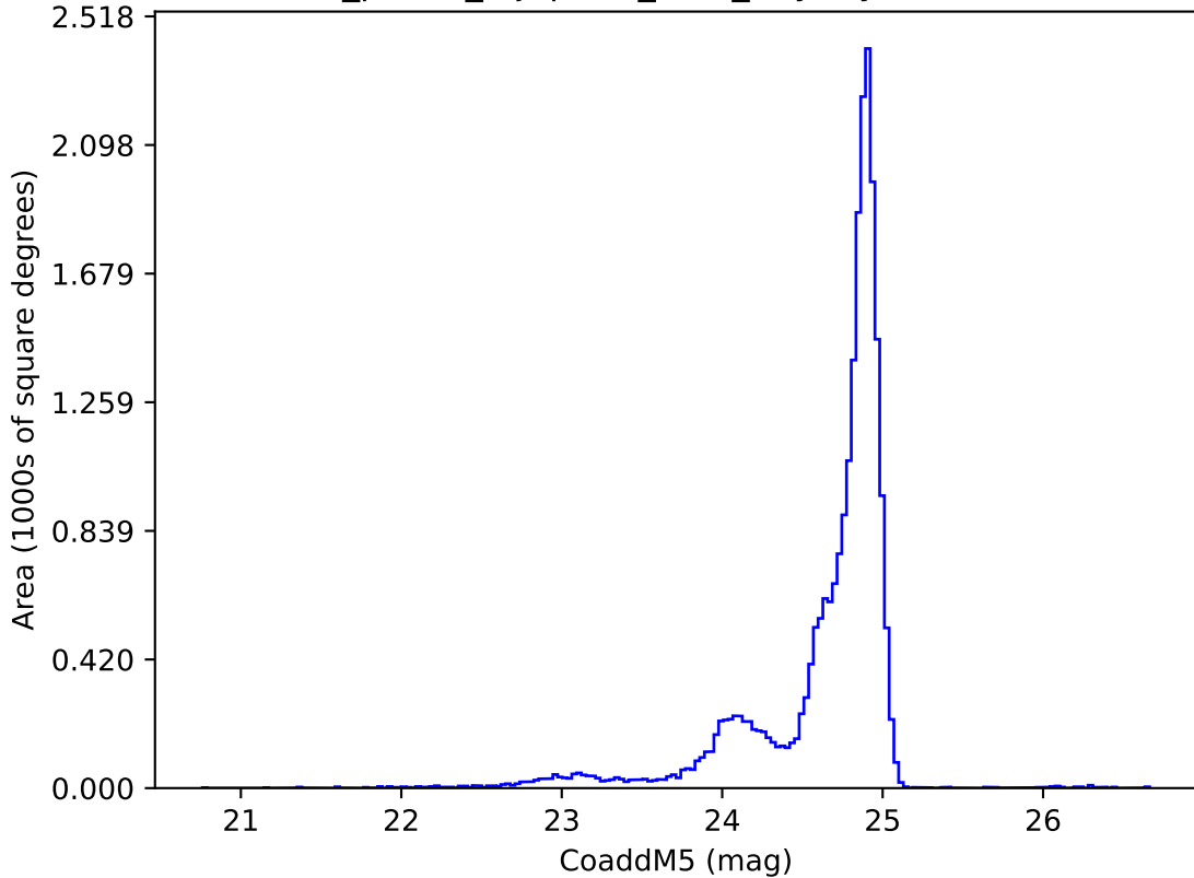
roll_pause_mjdp270_v3.4_10yrs y: CoaddM5
